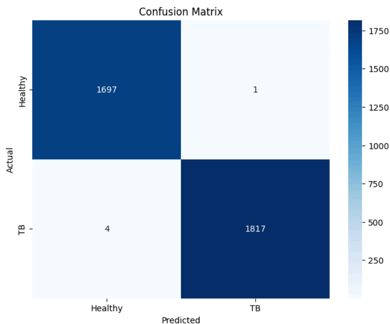
Confusion matrix of train dataset
