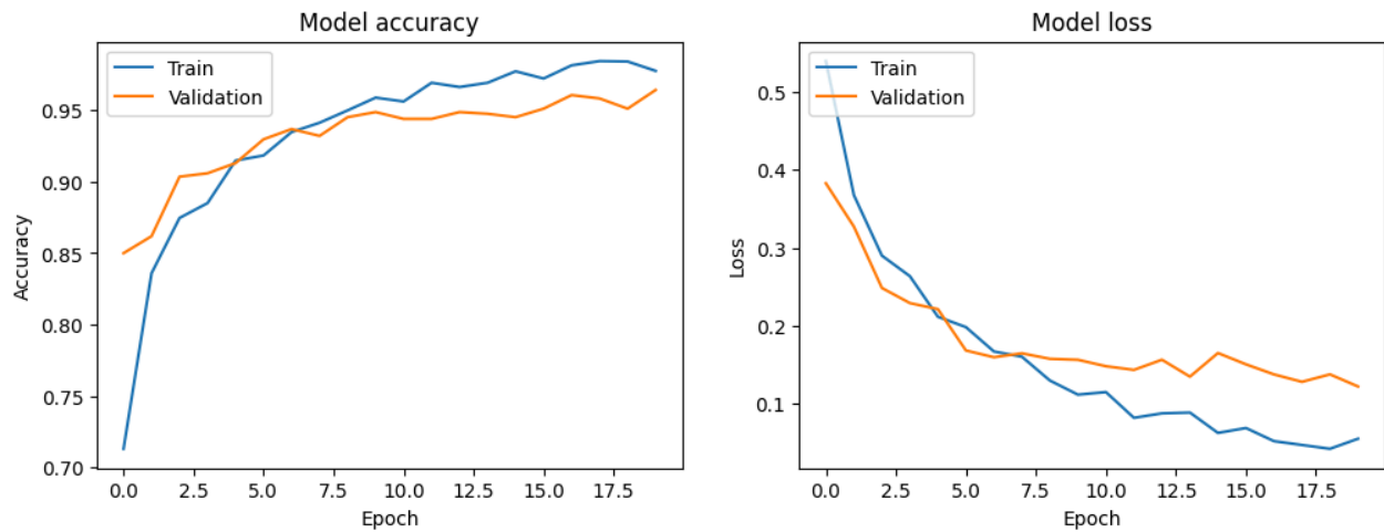
Accuracy and loss curve between train and validation
